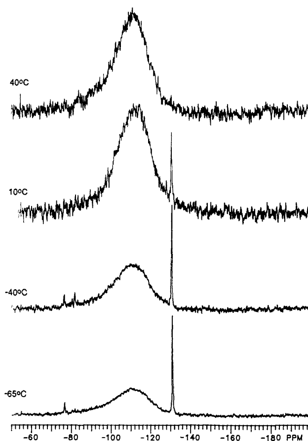
Figure 1. Variable temperature ^{29}Si[^1H] NMR spectra of an equimolar mixture of Si(OEt)_4 , KOEt , and 18-crown-6 in toluene solution.
