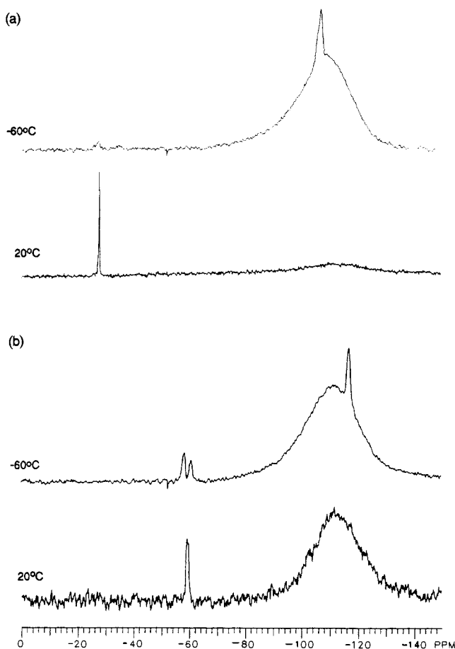
Figure 2. Variable temperature ^{29}\text{Si}\{^1\text{H}\} NMR spectra of equimolar mixtures in toluene solutions of (a) \text{Ph}_2\text{Si}(\text{OCH}_2\text{CF}_3)_2 , \text{K}(\text{OCH}_2\text{CF}_3) , and 18-crown-6 and (b) \text{vinylSi}(\text{OEt})_3 , KOEt, and 18-crown-6.
