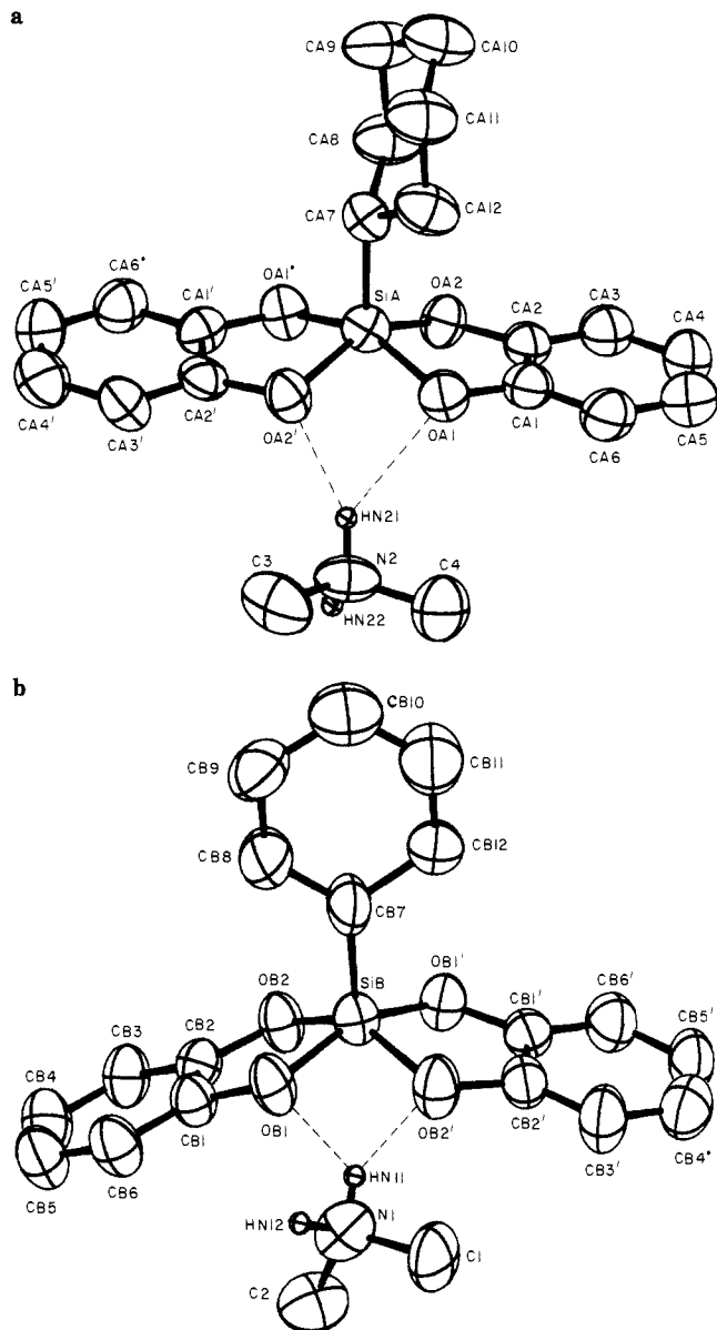
Figure 6. ORTEP plot of the asymmetric unit in [(C_6H_4O_2)_2SiC_6H_{11}][Me_2NH_2] , 3 , with thermal ellipsoids at the 50% probability level. Primed atoms are not symmetry related to unprimed ones. All but the amino hydrogen atoms are omitted for purposes of clarity: (a) showing one independent cation-anion pair and (b) showing the second independent cation-anion pair.
