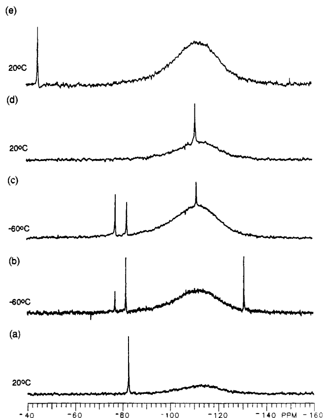
Figure 3. ^{29}\text{Si}\{^1\text{H}\} NMR spectra in toluene solutions of (a) \text{Si}(\text{OEt})_4 at 20^\circ\text{C} , (b) an equimolar mixture of \text{Si}(\text{OEt})_4 , KOEt, and 18-crown-6 at -60^\circ\text{C} , (c) the reaction mixture in (b) at -60^\circ\text{C} to which an equimolar amount of pinacol was added, (d) the bis(pinacolato), \text{Si}(\text{O}_2\text{C}_2\text{Me}_4)_2 , at 20^\circ\text{C} , and (e) \text{Si}(\text{O}_2\text{C}_2\text{Me}_4)_2 from (d) to which equimolar portions of KOEt and 18-crown-6 were added. The latter spectrum was the same at 20^\circ\text{C} and -60^\circ\text{C} .
