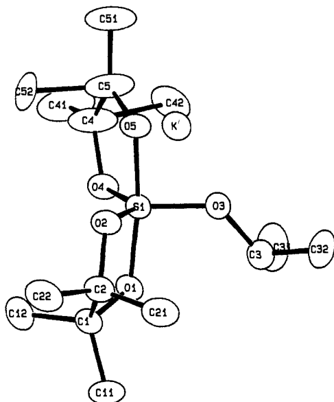
Figure 4. ORTEP plot of the anion and the potassium atom in [(\text{Me}_4\text{C}_2\text{O}_2)_2\text{SiO-}i\text{-Pr}][\text{K},18\text{-c-6}] , 1 , with thermal ellipsoids at the 30% probability level. Only one set of positions for the disordered C42 and C52 is shown. The potassium atom is related to that in the coordinate list by 1.5 - x, y - 1/2, 1/2 - z . Hydrogen atoms are omitted for clarity.
