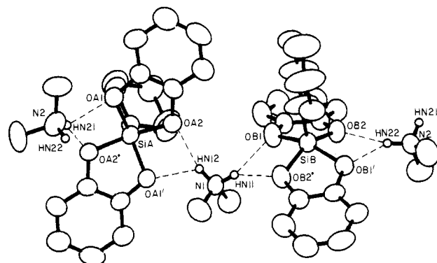
Figure 7. ORTEP plot of the asymmetric unit in [(C_6H_4O_2)_2SiC_6H_{11}][Me_2NH_2] , 3 , showing the hydrogen bonding interactions (dashed lines). A symmetry-related cation ( 1-x, y-1/2, 1.5-z ) is included at the right of the figure to show the propagation of the hydrogen-bonded chains.
